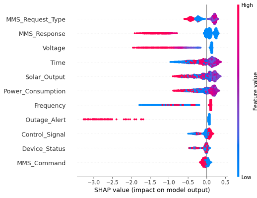
Fig. 3. Feature selection for ML model training.
