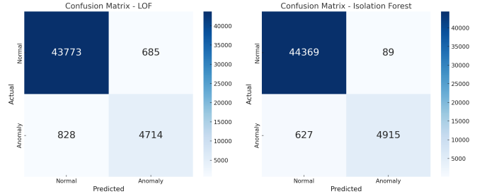
Fig. 4. Confusion Matrix for Local Outlier Factor &amp; Isolation Forest.
